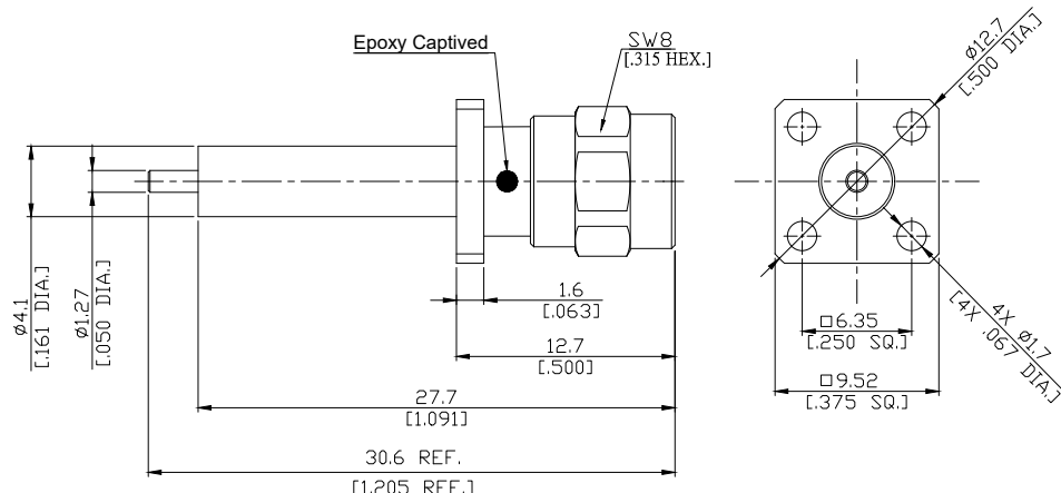
Mounting Dimensions
