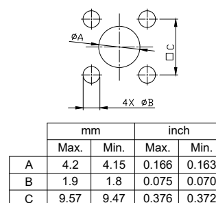
Mounting Dimensions
